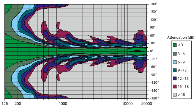
Vertical radiation pattern 3 x SEQUENZA 5 W, 6° splayed
