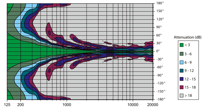
Vertical radiation pattern 3 x SEQUENZA 5 W, 3° splayed
