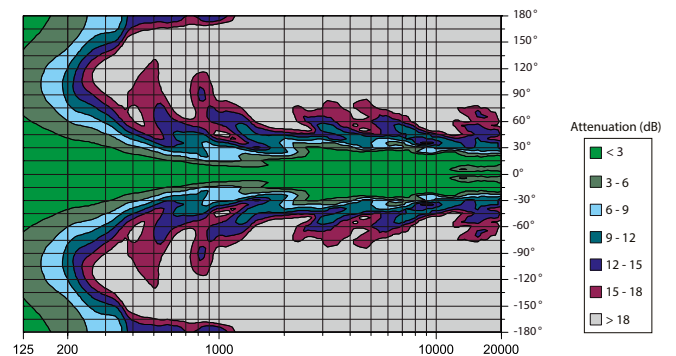
Vertical radiation pattern 3 x SEQUENZA 5 W, 15° splayed
