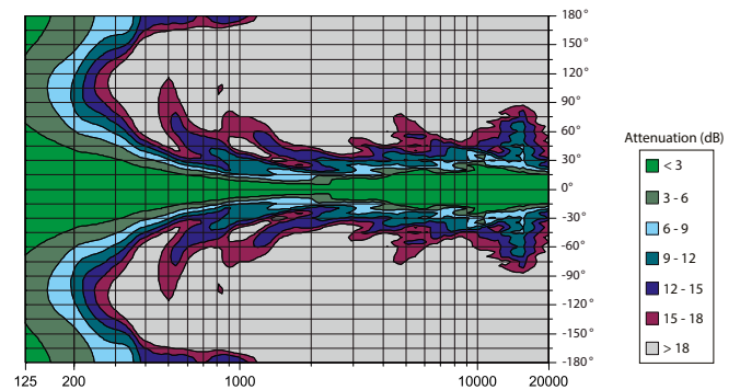
Vertical radiation pattern 3 x SEQUENZA 5 W, 9° splayed
