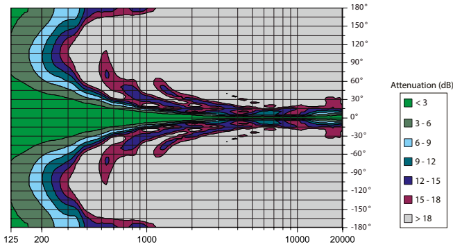
Vertical radiation pattern 3 x SEQUENZA 5 W, 0° splayed
