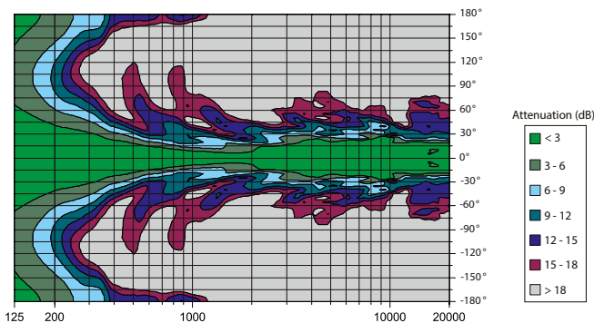
Vertical radiation pattern 3 x SEQUENZA 5 W, 12° splayed
